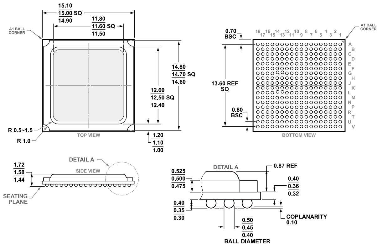
COMPLIANT TO JEDEC STANDARDS MO-275-KKAB-1 Figure 44. 324-Ball Ball Grid Array, Thermally Enhanced [BGA_ED] (BP-324-3) Dimensions Shown in Millimeters
