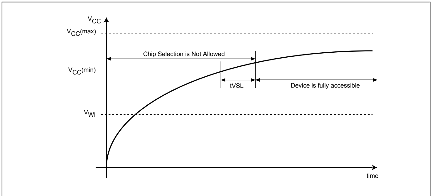
Figure 79. Power-up Timing
