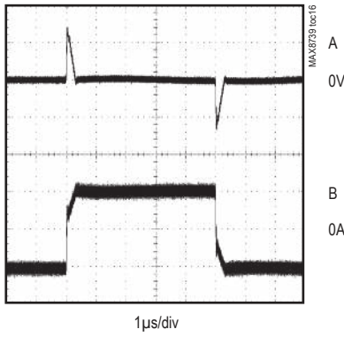
A: OUTPUT VOLTAGE, AC-COUPLED, 2V/div B: OUTPUT CURRENT, 50mA/div
