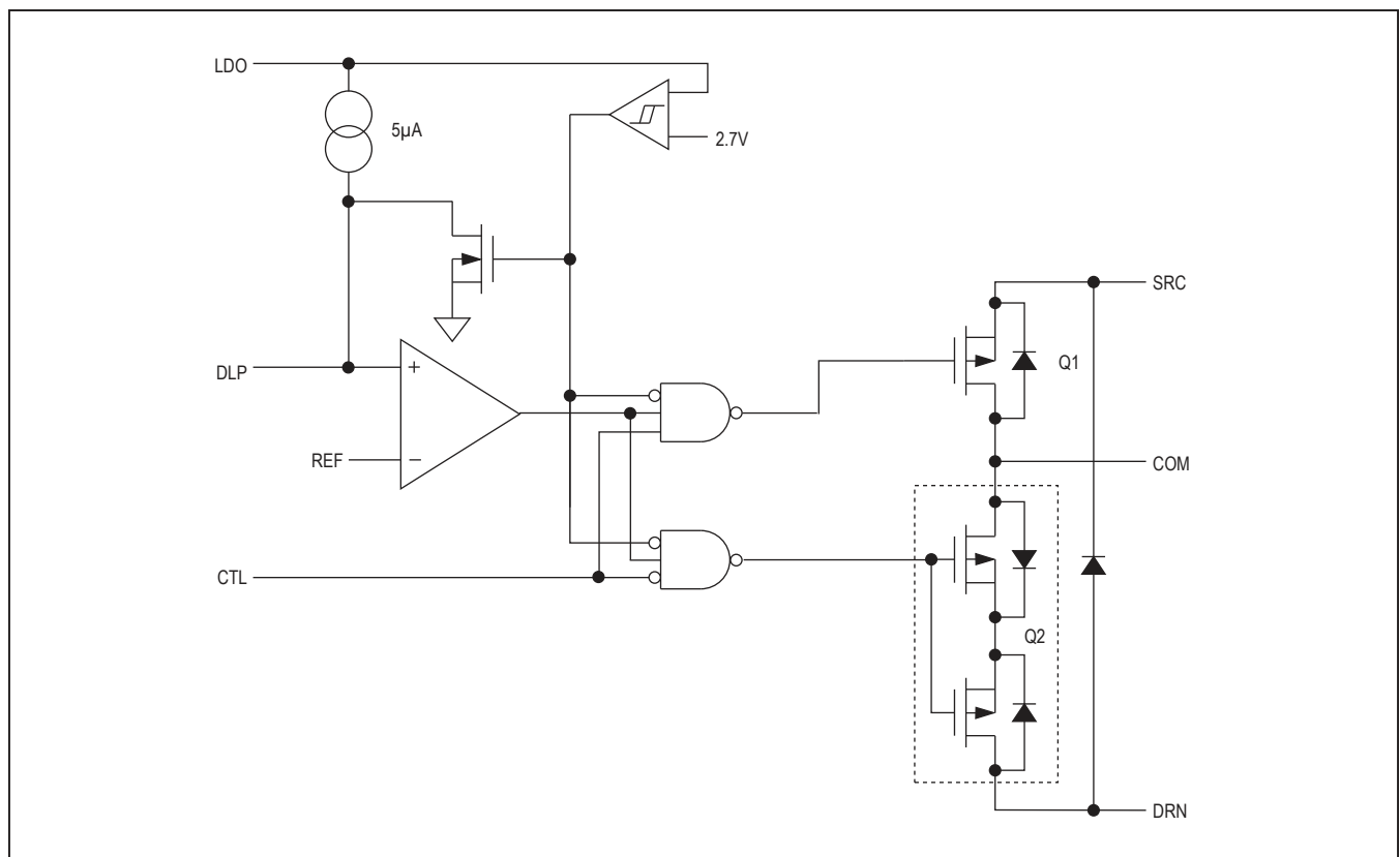
Figure 4. Switch Control
