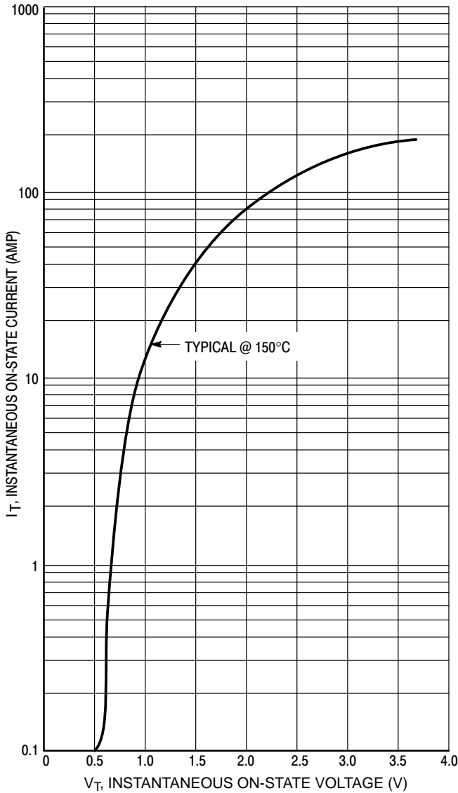
Figure 3. On-State Characteristics
