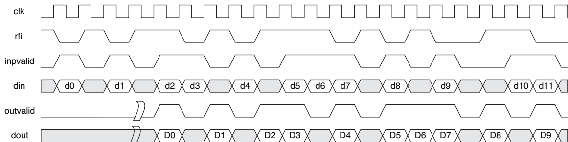
Figure 2-9. Single Channel, Single Rate FIR Filter with Gaps in Input
