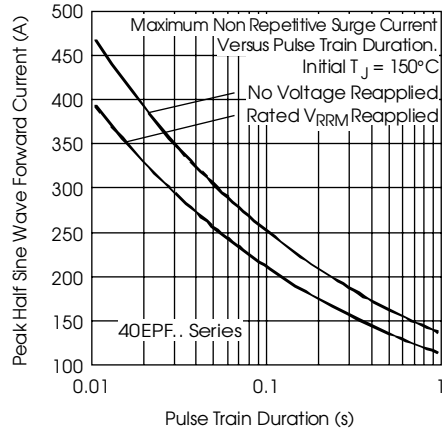
Fig.6-Maximum Non-Repertitive Surge Current
