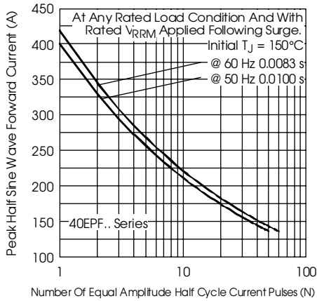
Fig.5-Maximum Non-Repertitive Surge Current
