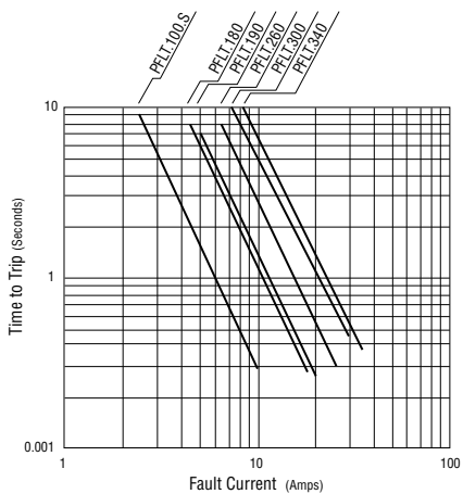
Typical Time to Trip at 23°C
