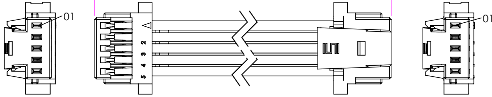
FIG 2 S1SS-05-XXX-XX-XX.XX-L1 SHOWN (DIFFERENT AS SHOWN, OTHERWISE SAME AS FIG 1)
