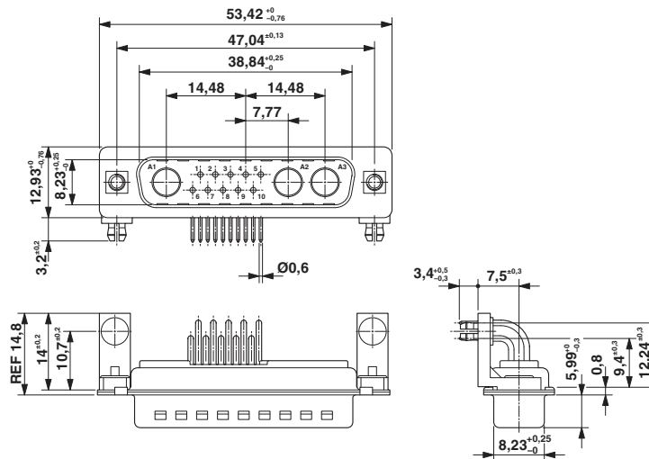
Dimensioned drawing
