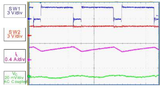
Figure 15. Buck region operation (PWM mode)
