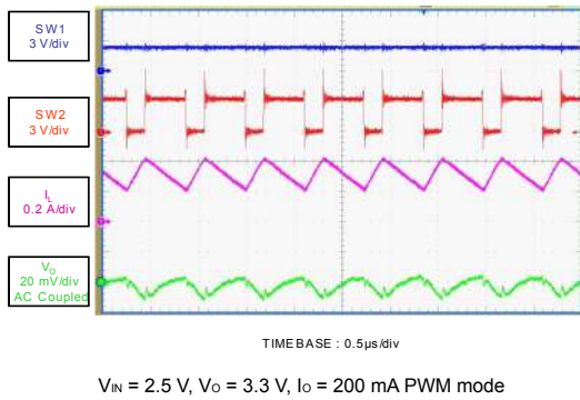
Figure 10. Boost region operation I_O = 200 mA
