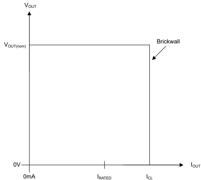
Figure 7-1. Current Limit
