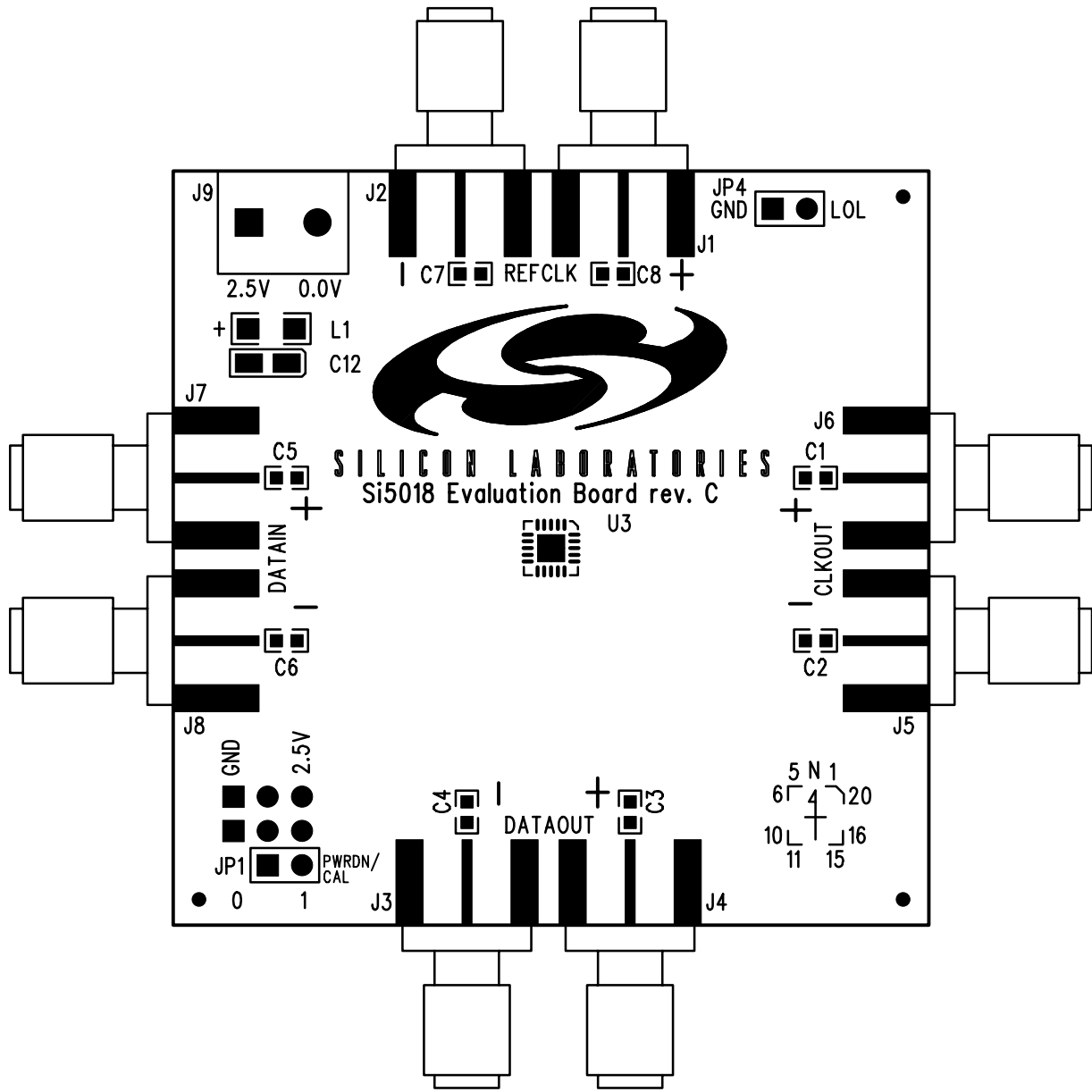
Figure 3. Si5018 Silkscreen
