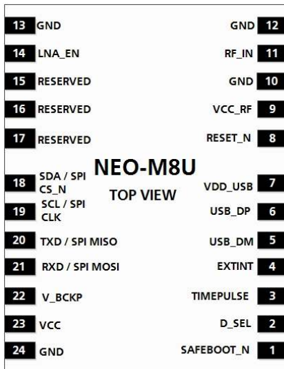
Figure 2: Pin assignment
