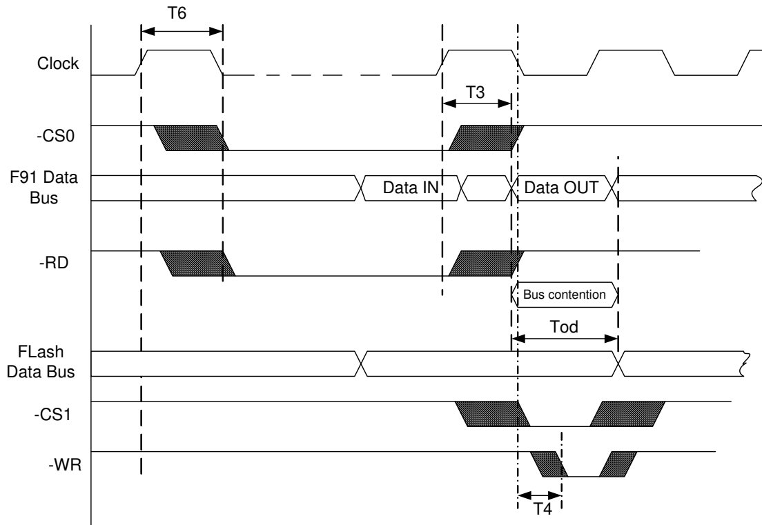
Figure 4. Bus Contention without the eZ80Acclaim! TM /eZ80AcclaimPlus! TM Ethernet Module: Fast Buffer Feature
