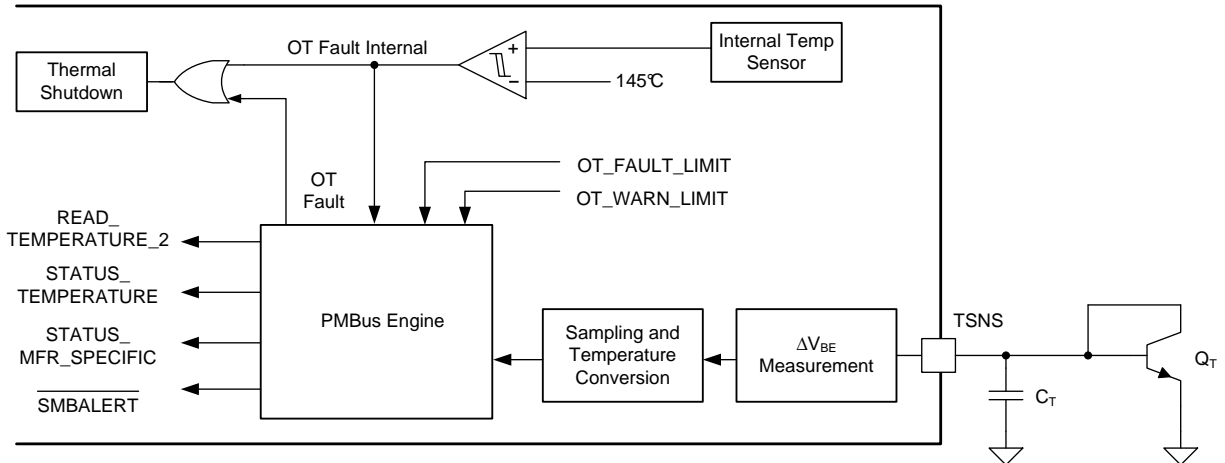
Figure 27. Over-Temperature Protection
