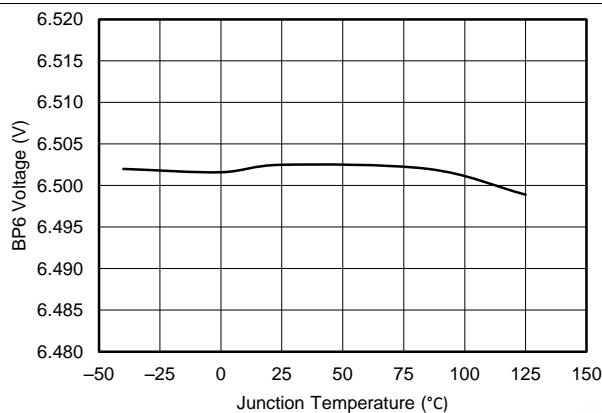
Figure 5. BP6 Voltage vs. Junction Temperature
