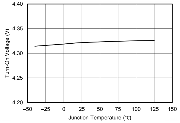
Figure 8. Turn-On Voltage vs. Junction Temperature
