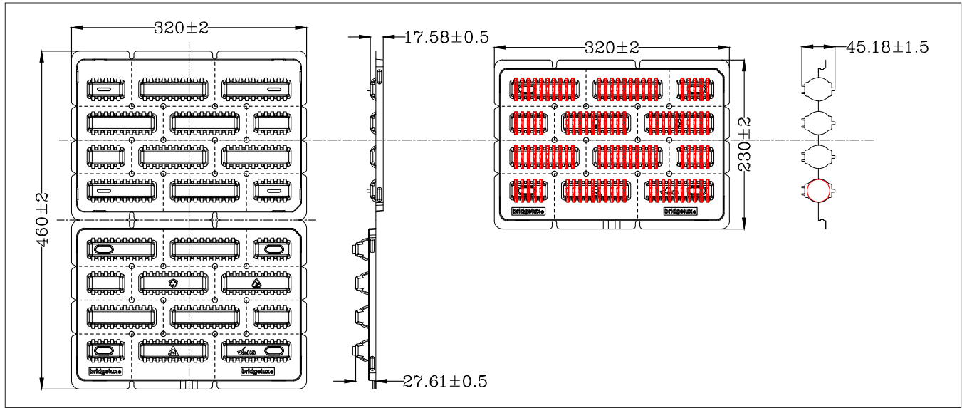
Figure 23: Packaging Specifications
