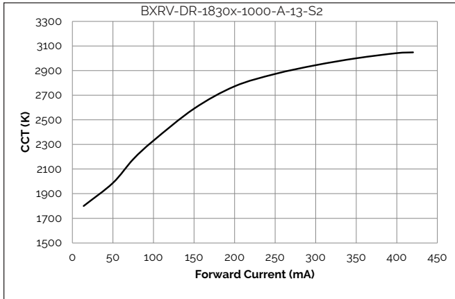
Figure 7: 6W CCT vs. Forward Current, T_c=25^\circ\text{C}
