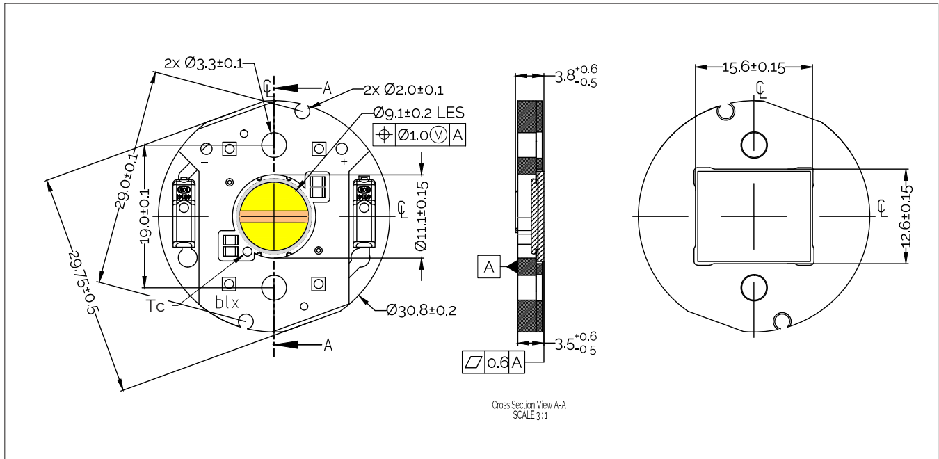
Figure 21: Mechanical Drawing Specifications
