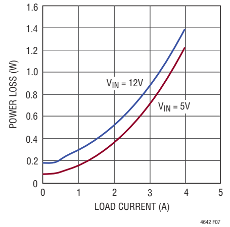
Figure 8. 3.3V Loss
