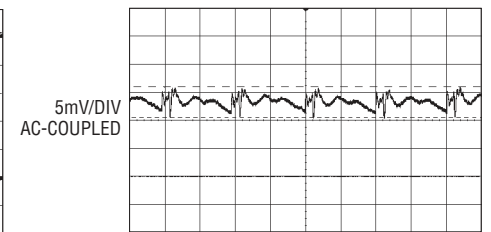
Output Ripple
