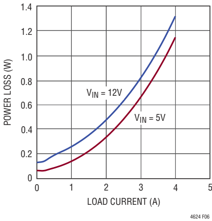
Figure 6. 1.0V Loss
