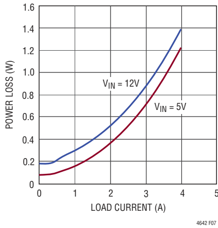
Figure 7. 1.5V Loss
