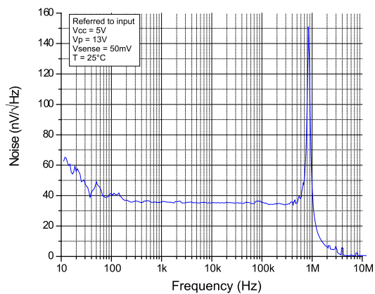
Figure 15: Noise level
