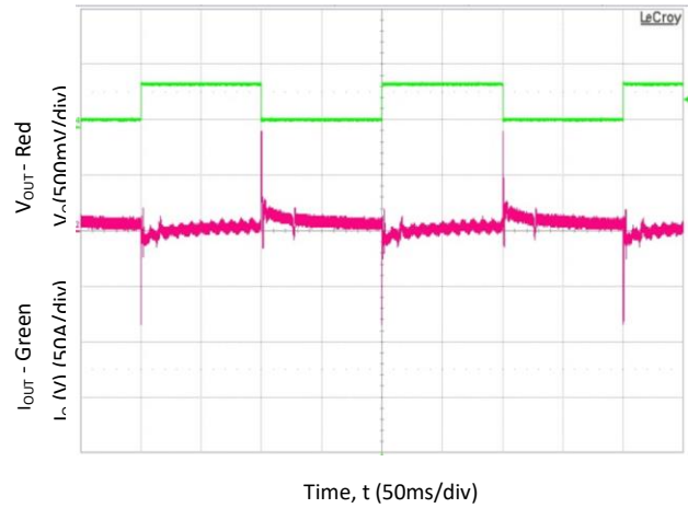
Figure 8. Transient response 52V DC load step 10 – 60%, Slew rate: 1A/ \mu s, V_{IN} = 230V AC .
