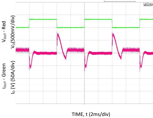
Figure 7. Transient response 52V DC load step 10 – 60%, Slew rate: 1A/ \mu s, V_{IN} = 230V AC
