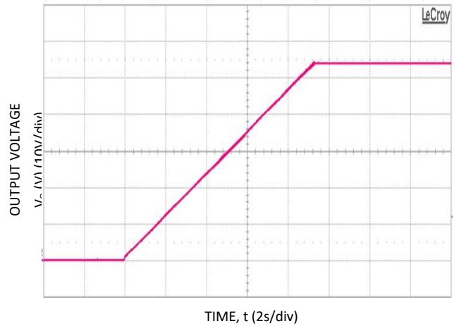
Figure 10. 52V DC soft start, full load, V_{IN} = 230V AC - RS485 mode with 4700 \mu f external capacitance.
