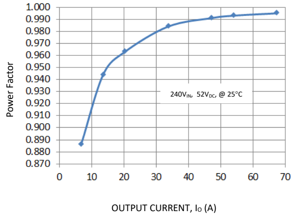
Figure 2. Power Factor versus Output Current
