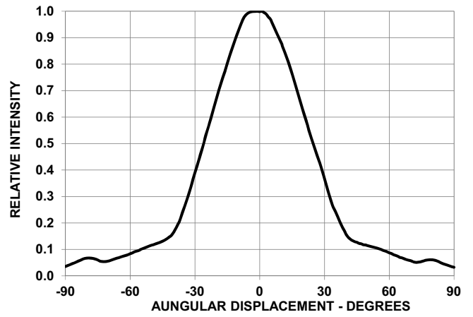
Figure 7: Radiation Pattern
