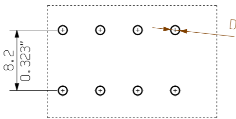
HOLE PATTERN
