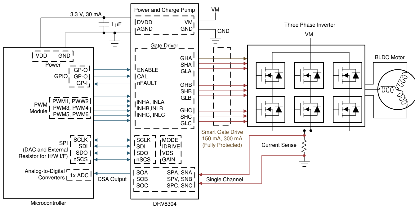
Figure 57. Alternative Application Schematic
