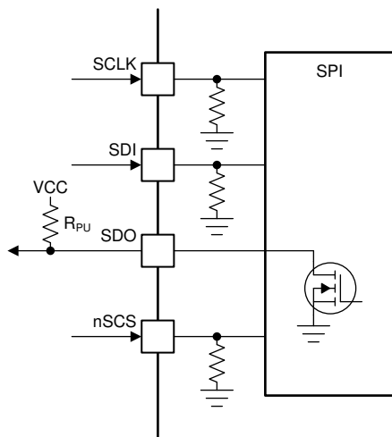
Figure 17. SPI
