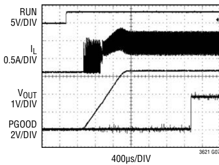
Soft-Start Operation
