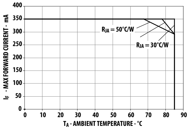
Figure 5. Maximum forward current vs. ambient temperature for AlInGaP Derated based on T_{jMAX} = 110^{\circ}C , R_{\theta JA} = 30^{\circ}C/W / 40^{\circ}C/W and 50^{\circ}C/W
