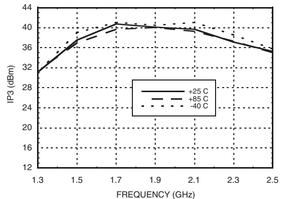
Output IP3 vs. Temperature, Vs= 5V
