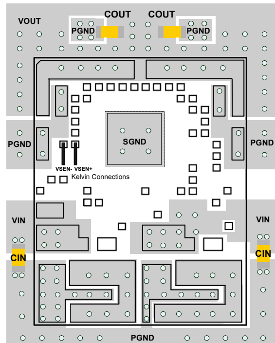
FIGURE 27. RECOMMENDED LAYOUT
