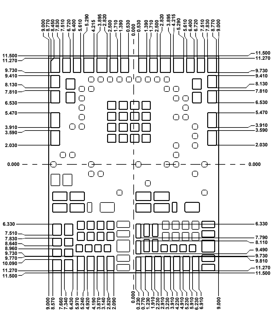
STENCIL OPENING EDGE POSITION - 1
