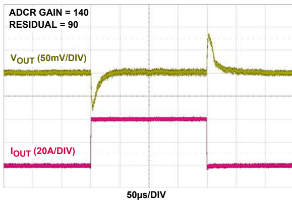
FIGURE 14. 12V IN TO 1V OUT TRANSIENT RESPONSE, f_{SW} = 300kHz , C_{OUT} = 14 \times 100\mu F CERAMIC + 6x470µF POSCAP
