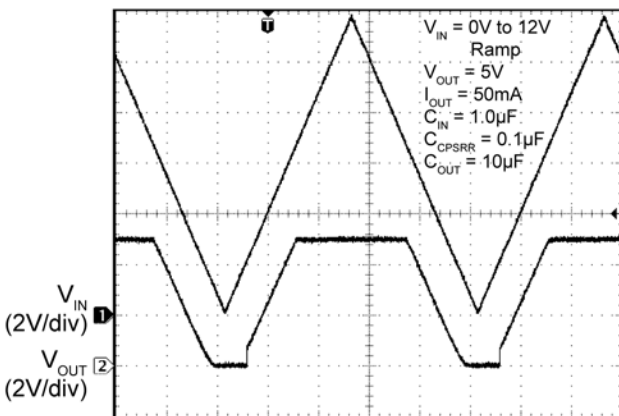
Time (200ms/div)
