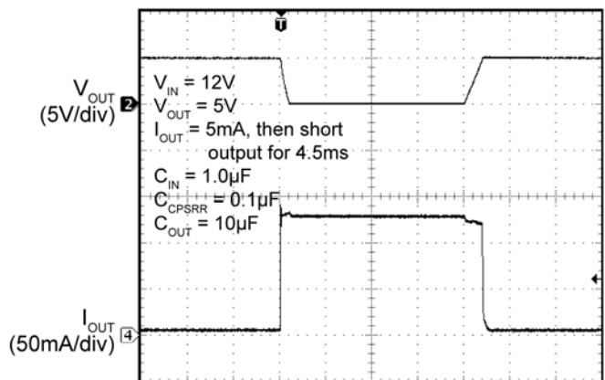
Time (1.00ms/div)
