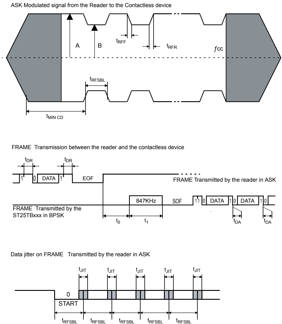
Figure 44. ST25TB512-AT synchronous timing, transmit and receive
