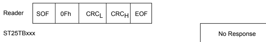
Figure 30. Completion frame exchange between reader and ST25TB512-AT
