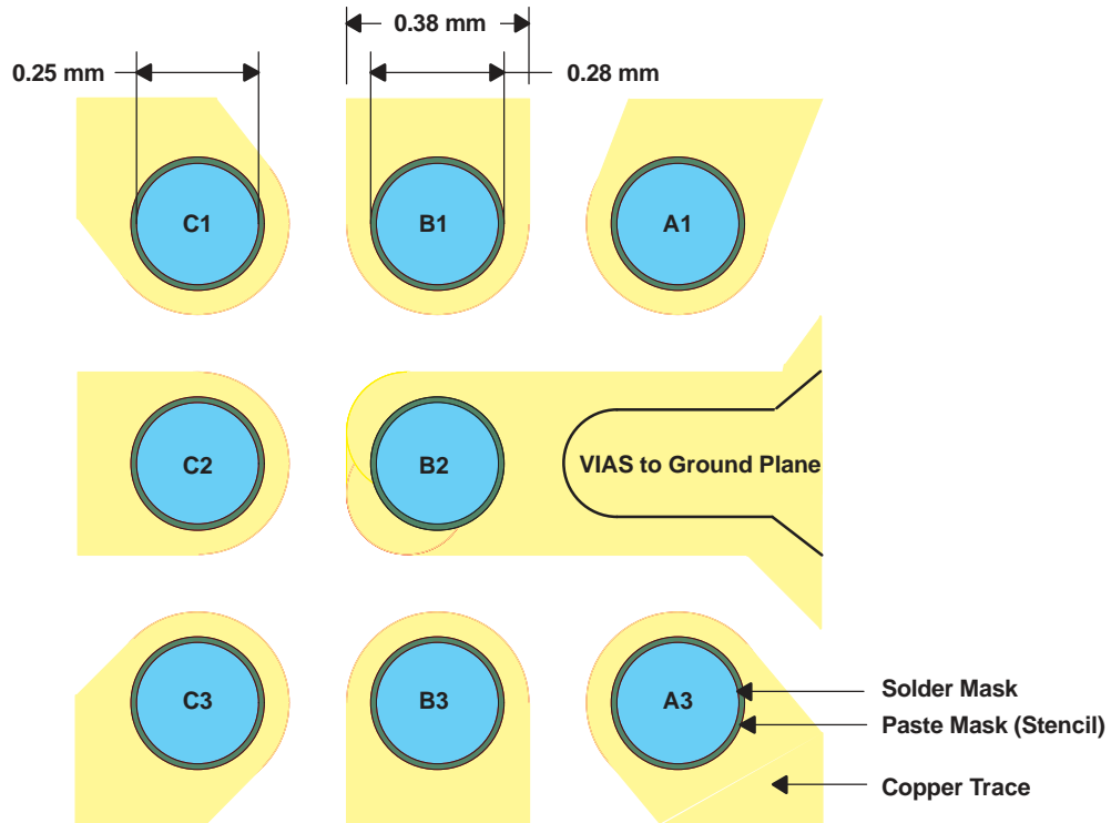
Figure 34. MicroStar Junior™ BGA Recommended Layout
