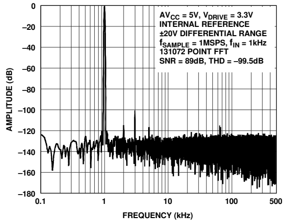
Figure 12. FFT, \pm 20\text{ V} Differential Range, High Bandwidth Mode
