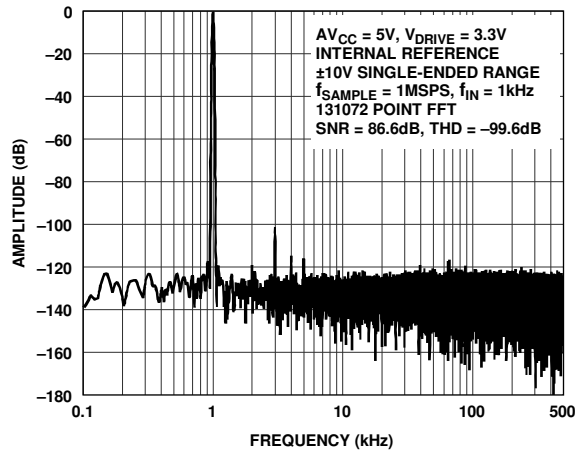
Figure 13. FFT, \pm 10\text{ V} Single-Ended Range, High Bandwidth Mode
