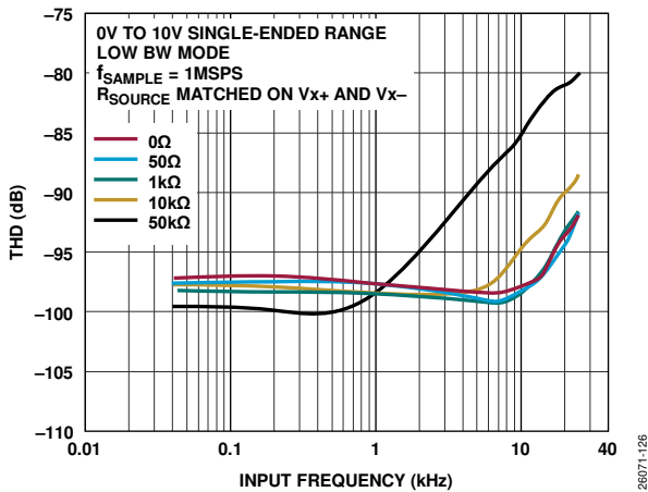
Figure 35. THD vs. Input Frequency for Various Source Impedances, 0 V to 10 V Single-Ended Range, Low Bandwidth Mode
