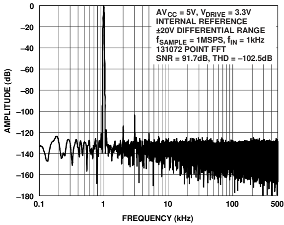
Figure 9. Fast Fourier Transform (FFT), \pm 20\text{ V} Differential Range, Low Bandwidth Mode
