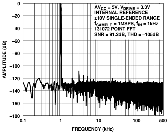
Figure 10. FFT, \pm 10\text{ V} Single-Ended Range, Low Bandwidth Mode
