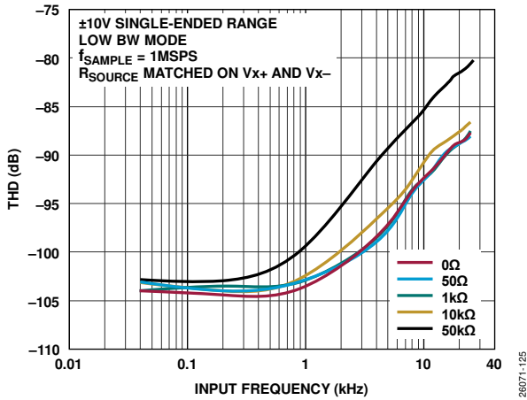
Figure 34. THD vs. Input Frequency for Various Source Impedances, \pm 10 V Single-Ended Range, Low Bandwidth Mode
