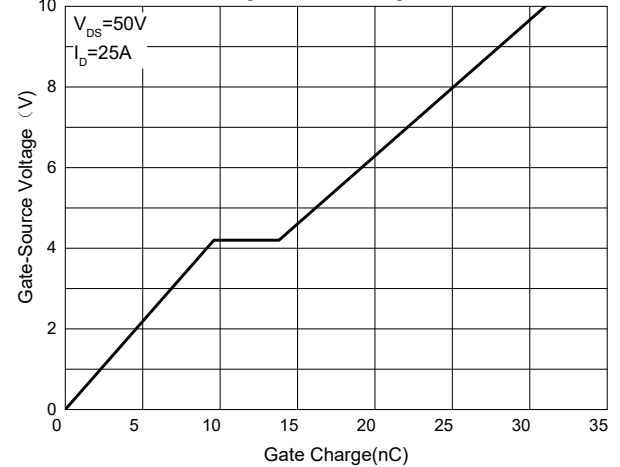
Fig. 6 - Gate Charge
