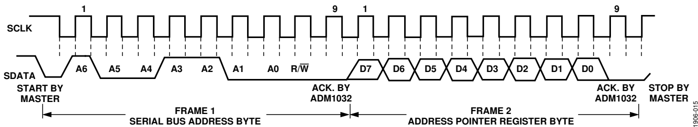
Figure 15. Writing to the Address Pointer Register Only
