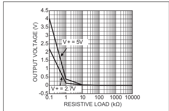
FIGURE 3-12: Output Voltage Swing vs. Resistive Load (Sink).
