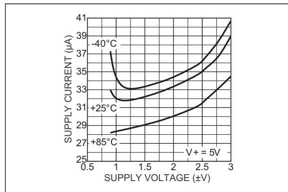
FIGURE 3-5: Supply Current vs. Supply Voltage.
