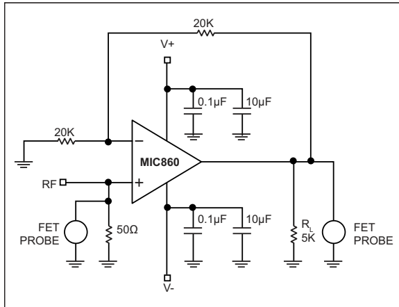
FIGURE 2-2: Test Circuit 2, A_V = 2 .
