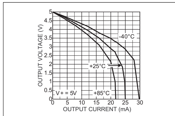
FIGURE 3-6: Output Voltage vs. Output Current (Source).
