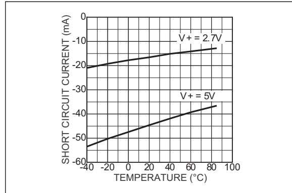
FIGURE 3-4: Short-Circuit Current (Sink) vs. Temperature.
