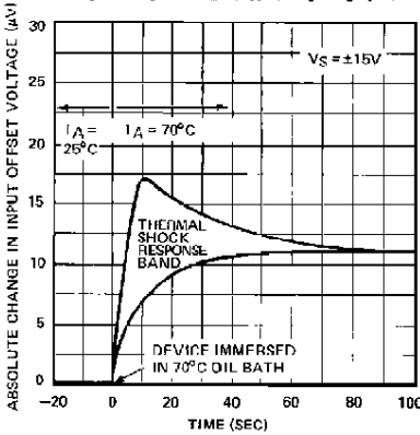
OFFSET VOLTAGE CHANGE DUE TO THERMAL SHOCK
