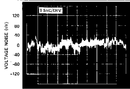
0.1Hz TO 10Hz PEAK-TO-PEAK NOISE
