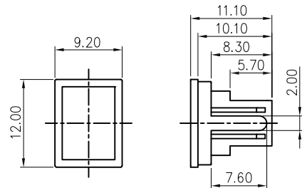
DUST CAP DRAWING
