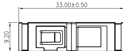
DRAWINGS WITH DUST CAPS
