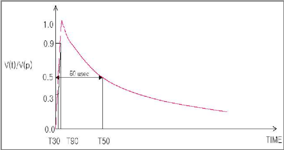
Figure 1. Combination wave, Open Surge Voltage (IEC 61000-4-5)
