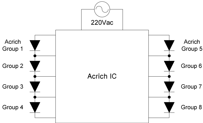
Circuit Diagram of Acrich 2
