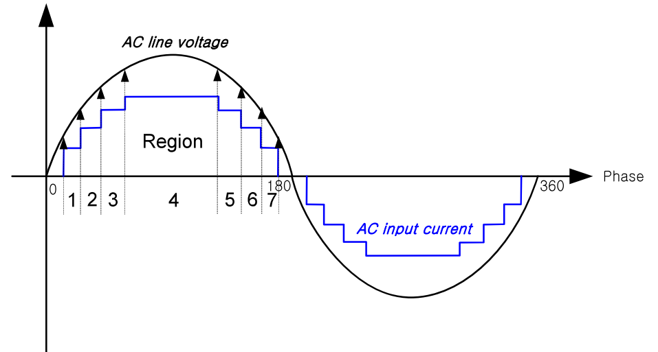
AC Input Current Wave ( = Acrich's Driving Current )
