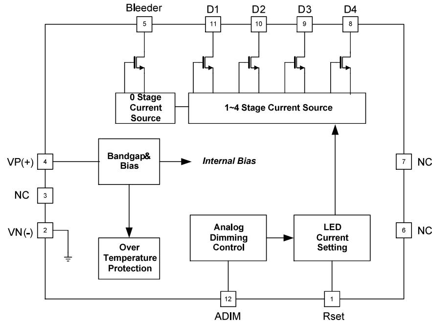
Figure. 3 Block Diagram
