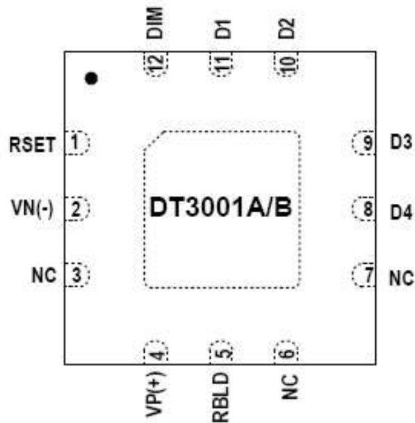
Figure. 2 Package – Top View
