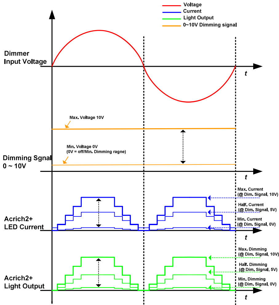
Figure 1. Analog Dimming Timing chart
