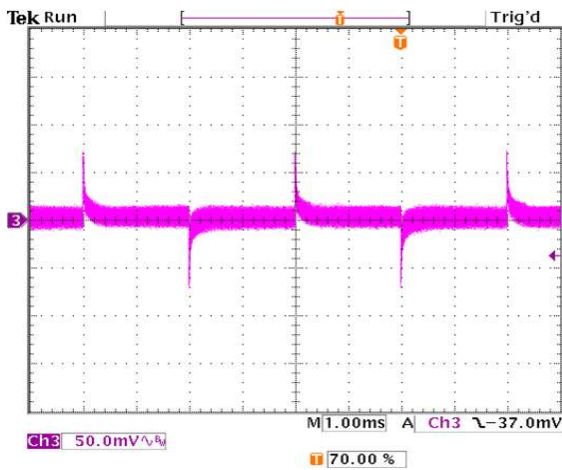
Figure 43. Transient Response with Regulation set to 0.0 mV/A
