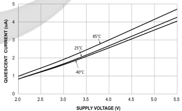
Figure 5. Quiescent Current vs. Supply Voltage
