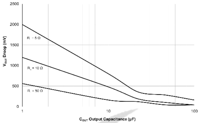
Figure 12. Output Voltage Droop at Switching Over from V_{IN1} (5 V) to V_{IN2} (3 V)
