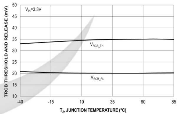
Figure 11. True Reverse Current vs. Temperature
