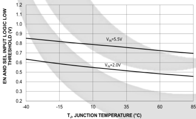
Figure 10. EN and SEL Input Logic Low Threshold vs. Temperature
