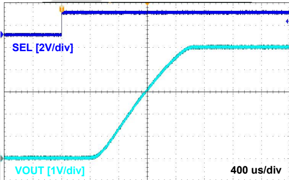
Figure 14. Turn-On Response
