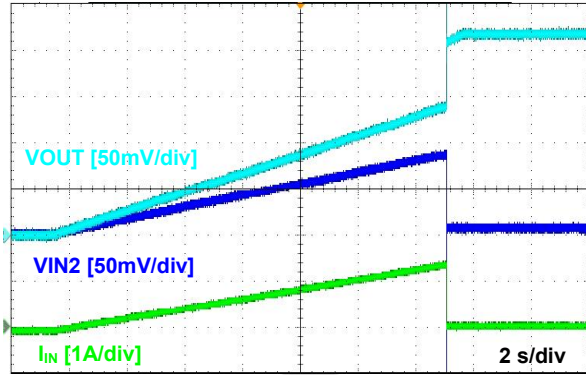
Figure 18. True Reverse Current Blocking on Each VIN VIN1 or VIN2=3.3 V, VOUT= From 3 V to 3.4 V, CIN=COUT=10 \mu F
