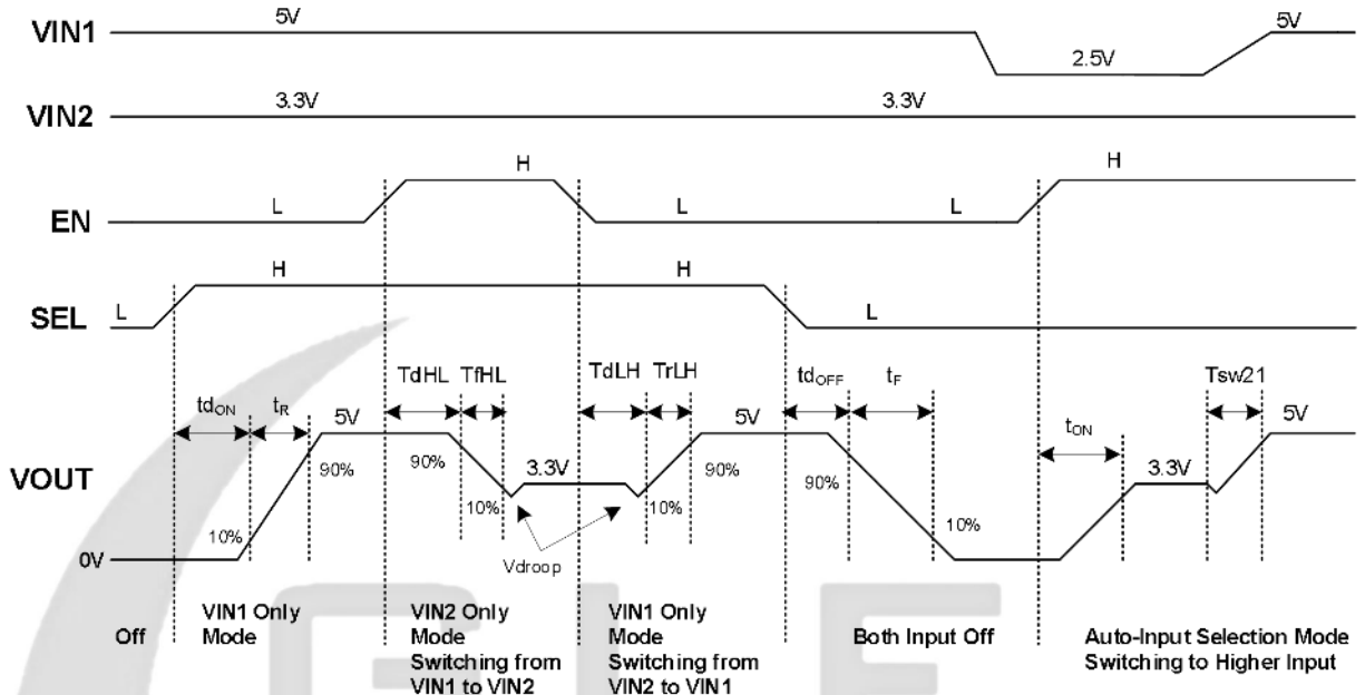
Figure 3. Timing Diagram
