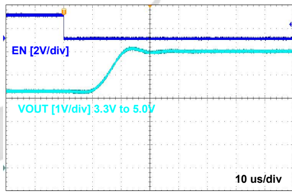
Figure 17. V_{OUT} Switchover 3.3 V_{IN} to 5 V_{IN}
