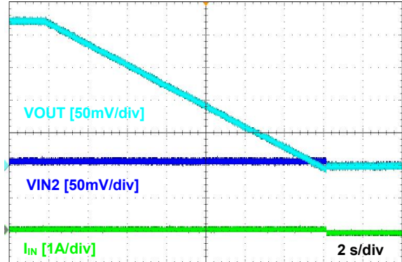
Figure 19. True Reverse Current Blocking Release VIN1 or VIN2=3.3 V, VOUT= From 3 V to 3.4 V, CIN=COUT=10 \mu F
