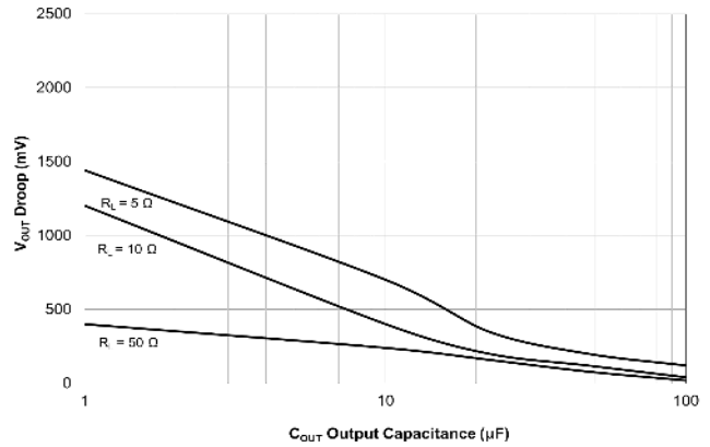
Figure 13. Output Voltage Droop at Switching Over from V_{IN2} (3 V) to V_{IN1} (5 V)
