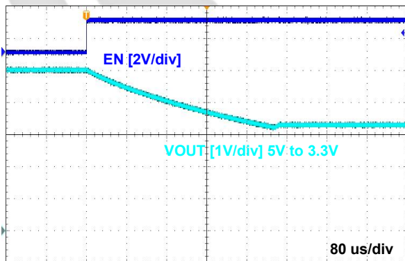
Figure 16. V_{OUT} Switchover from 5 V_{IN} to 3.3 V_{IN}
