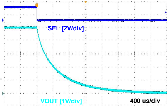
Figure 15. Turn-Off Response
