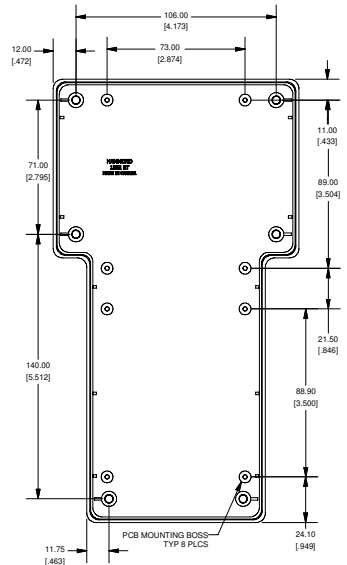
FRONT VIEW OF BOX
