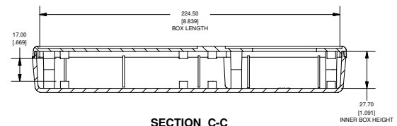
SECTION C-C SCALE 1 / 2
