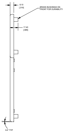
END VIEW OF ASSEMBLY
