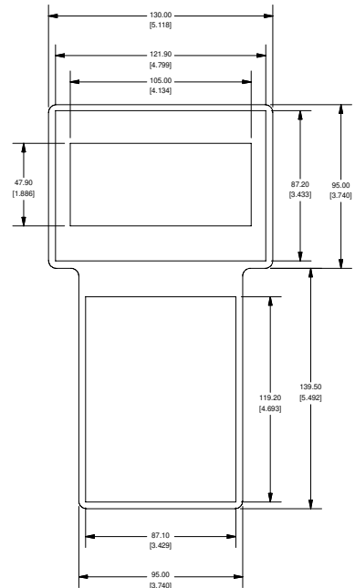
FRONT VIEW OF LID
