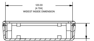
SECTION B-B SCALE 1 / 2
