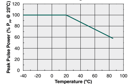
TVS Derating Curve
