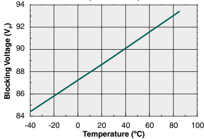
Blocking Voltage vs. Temperature (Pins 5 & 6)
