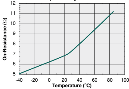
On-Resistance vs. Temperature ( I_F=1\text{mA} , I_L=50\text{mA} )
