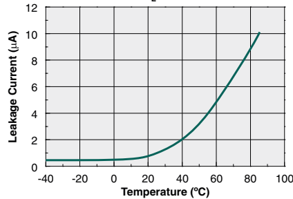
Leakage Current vs. Temperature Measured Between Pins 5 & 6 ( V_L=70\text{V} )
