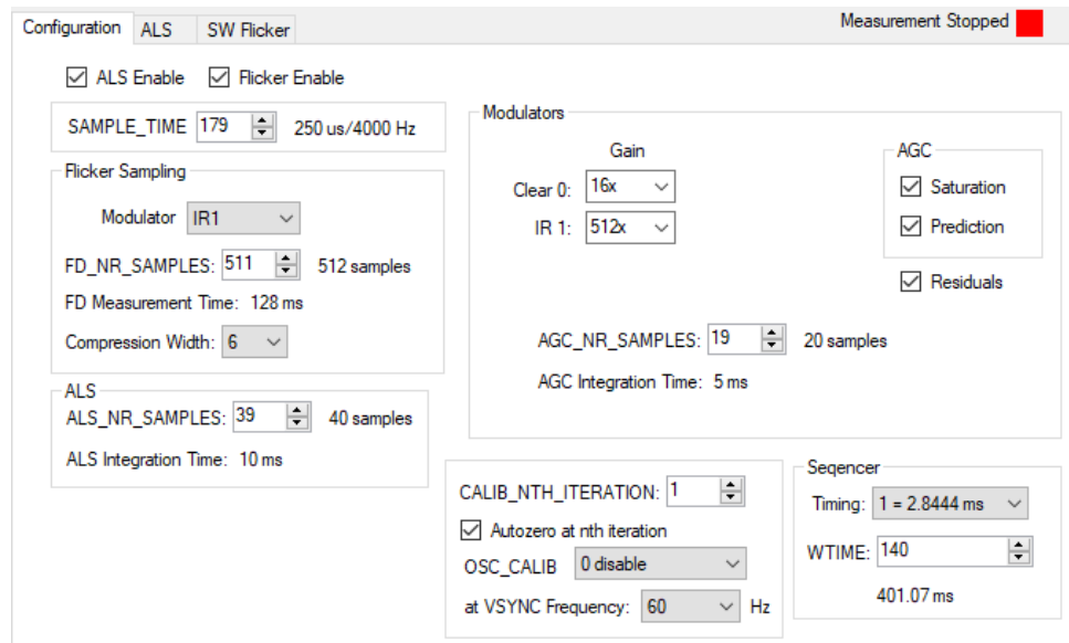
Figure 9 : Configuration Tab
