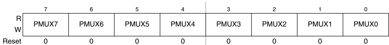
Figure 17-6. PIT Multiplex Register (PITMUX)
