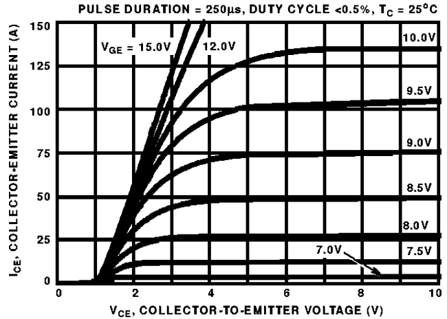
FIGURE 2. SATURATION CHARACTERISTICS
