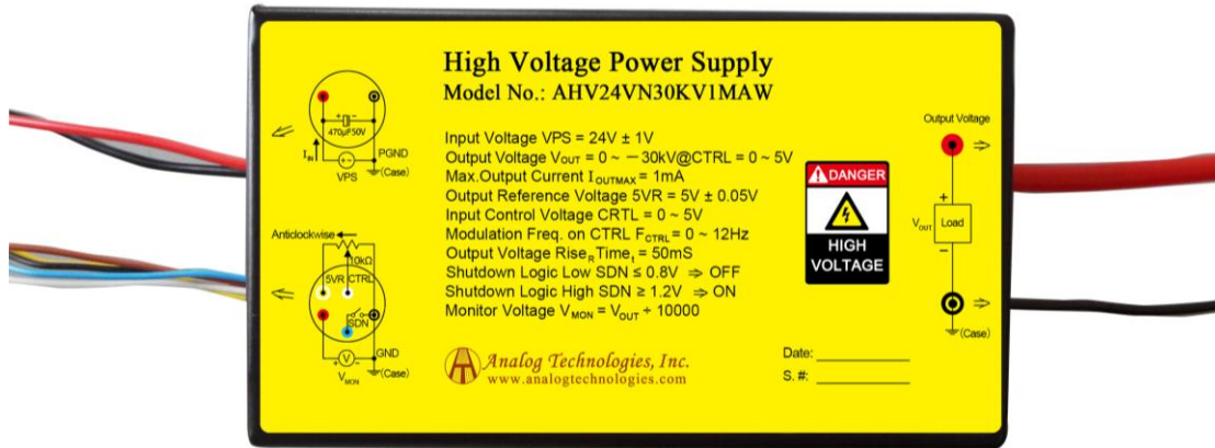
Figure 1. Physical Photo of AHV24VN30KV1MAW
