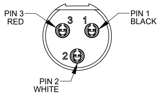
ST-603 FRONT MATING VIEW BOTH ENDS
