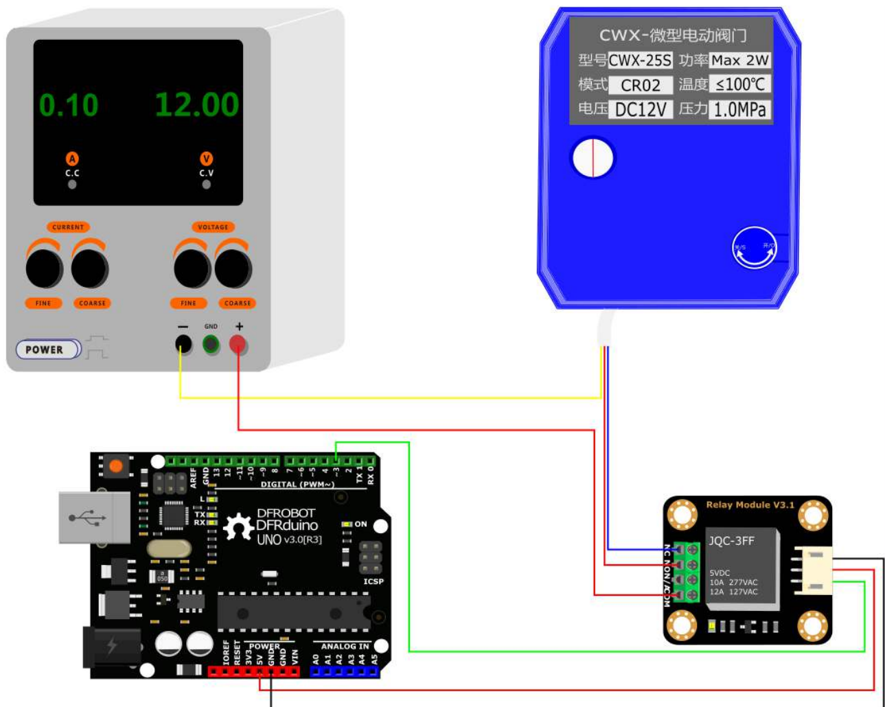
FIT0617-Arduino Connection Diagram
