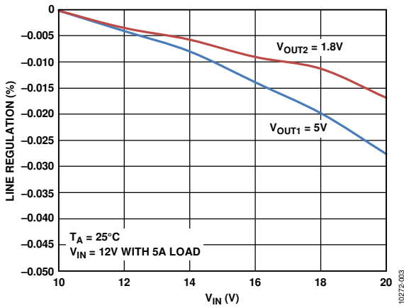
Figure 3. Line Regulation
