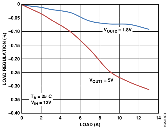
Figure 4. Load Regulation
