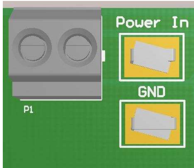
Figure 5. Power Input Terminal Block (P1)
