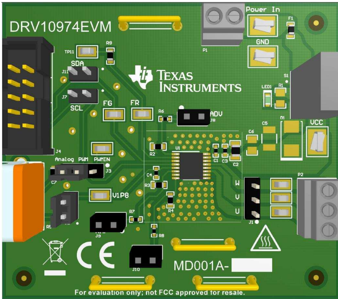
Figure 1. DRV10974 EVM
