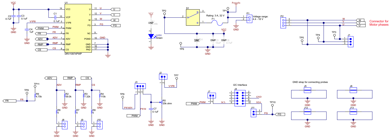
Figure 13. DRV10974 EVM Schematic
