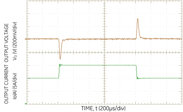
Figure 4. Transient Response to 1.0A/ \mu s Dynamic Load Change from 50% to 75% to 50% of full load.
