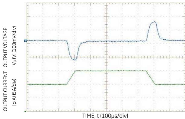
Figure 3. Transient Response to 0.1A/ \mu s Dynamic Load Change from 50% to 75% to 50% of full load.
