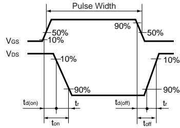
Fig.13 Switching Time Waveforms
