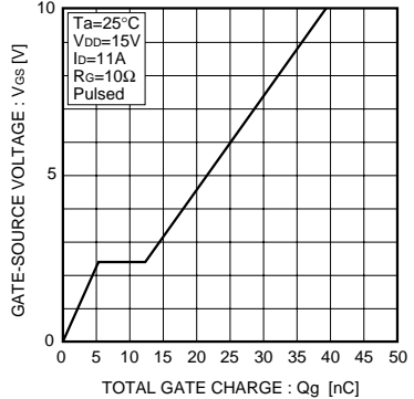
Fig.10 Dynamic Input Characteristics
